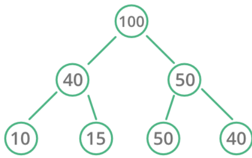
Max Heap
